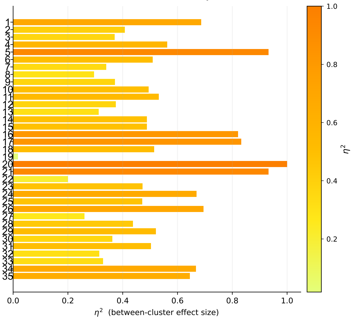
Feature discriminability
